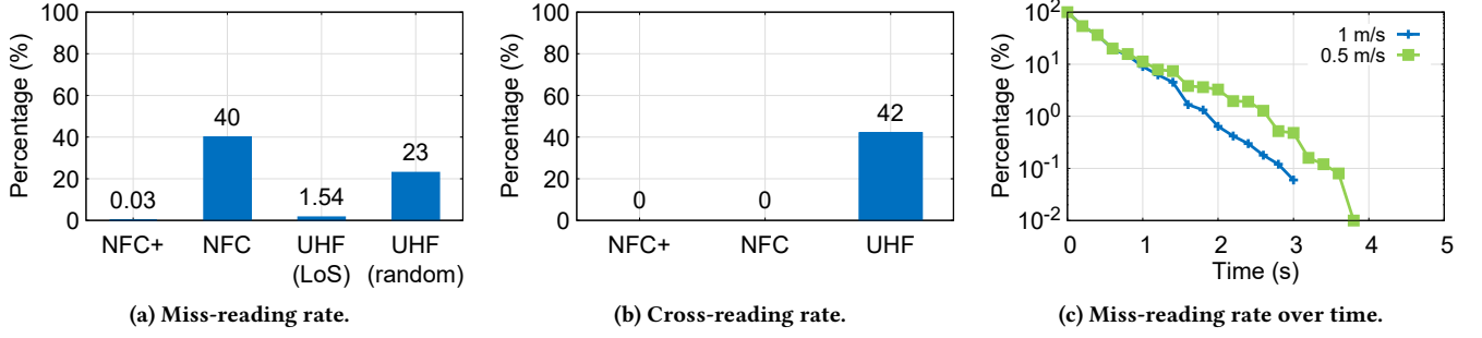
Figure 18: NFC+'s performance in a warehouse. Over 10k tags are used. NFC+ can read over 1-0.03%=99.97% desired tags and does not any undesired tags. In comparison, commercial NFC systems and UHF RFID suffers from severe miss-reading or cross-reading.
