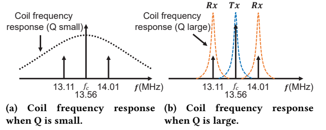
Figure 5: Frequency response of coils with different quality factors. To use high Q coils, we use different coils for transmission and reception. The TX coils are tuned to 13.56 MHz and the RX coils are tuned to 13.11 MHz or 14.01 MHz.
