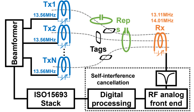
Figure 3: NFC+'s system overview
