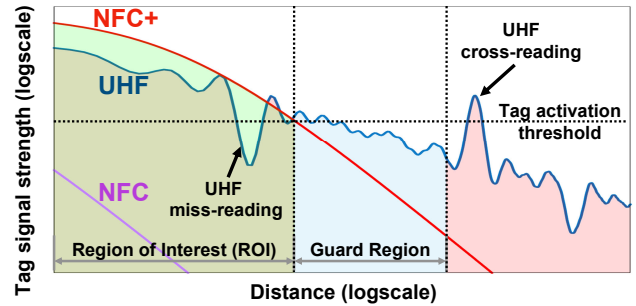
Figure 1: The propagation characteristics of the RF signal make UHF RFID unable to avoid miss-reading and cross-reading. In contrast, NFC+ leverages magnetic field to avoid miss-reading and cross-reading. Its operational range is significantly larger than NFC, which makes it suitable for logistics network applications.
