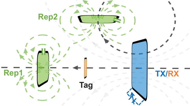
Figure 11: TX coil, mag-repeater placement and magnetic field line from TX coil and mag-repeater.
