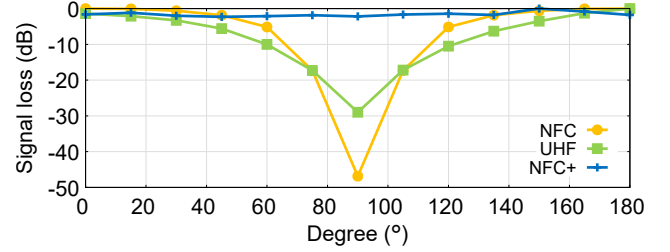
Figure 16: Performance of NFC+, state-of-the-art NFC, and UHF RFID with different tag orientations.
